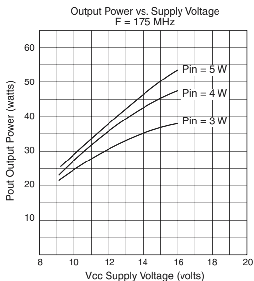
Figure 5. Power Output vs Supply Voltage (175 MHz)
